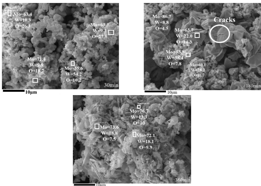
Fig. 11. EDAX analysis of the reduced sample \text{MoO}_3 -26.5wt% \text{WO}_3 at 700°C
