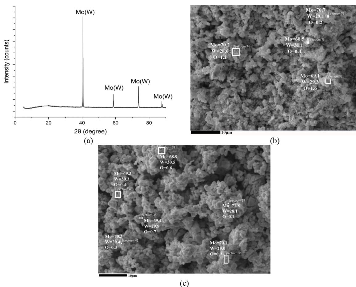
Fig. 16. X-ray pattern (b) EDAX analysis of reduced \text{MoO}_3 -26.5% \text{WO}_3 mixture by 600°C, 60 min + 600°C to 1050°C during 240 minutes + 1050°C, 180 min (optimum condition) (c) EDS analysis of the duplicate oxide sample reduced under optimal conditions
