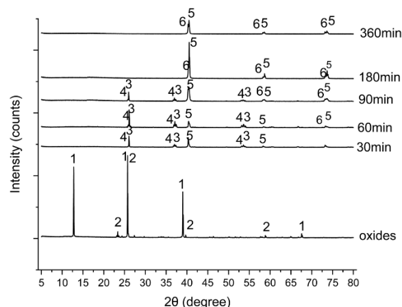
Fig. 6. XRD results of reduced \text{MoO}_3\text{-}26.5\text{WO}_3 at 800°C at different times (1: \text{MoO}_3 , 2: \text{WO}_3 , 3: \text{MoO}_2 , 4: \text{WO}_2 , 5: Mo, 6: W)
