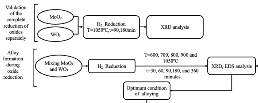
Fig. 2. Flowchart of the experimental procedure
