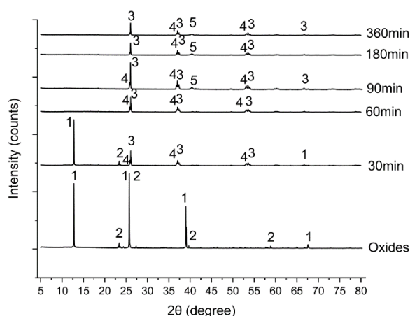
Fig. 4. XRD results of reduced MoO 3 -26.5WO 3 at 600°C at different times (1: MoO 3 , 2: WO 3 , 3: MoO 2 , 4: WO 2 , 5: Mo, 6: W)
