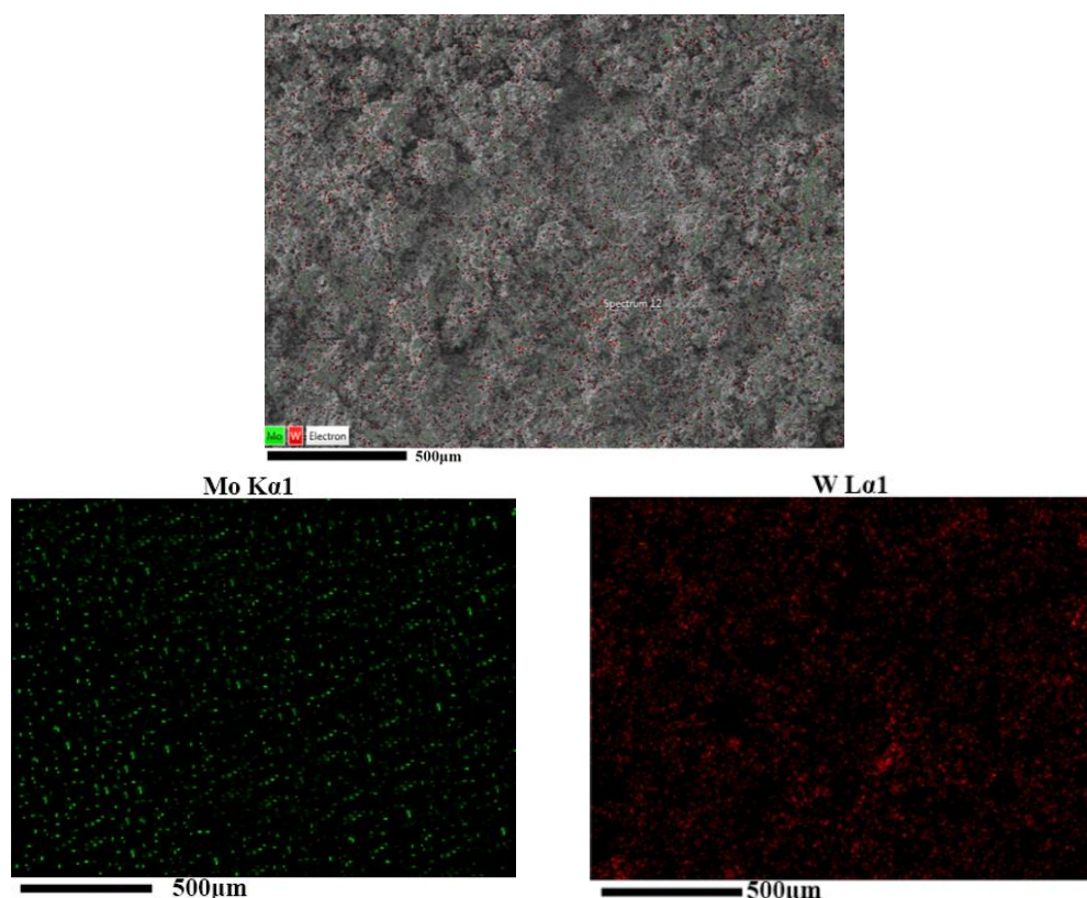
Fig. 17. elemental map of \text{MoO}_3 -26.5 wt.% \text{WO}_3 after reduction ( 600^\circ\text{C} , 60 min + 600^\circ\text{C} to 1050^\circ\text{C} during 240 minutes + 1050^\circ\text{C} , 180 min)
