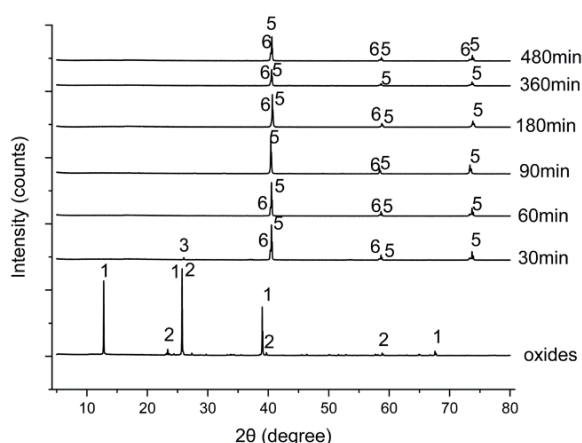
Fig. 8. XRD results of reduced \text{MoO}_3 -26.5 \text{WO}_3 at 1050°C at different times (1: \text{MoO}_3 , 2: \text{WO}_3 , 3: \text{MoO}_2 , 4: \text{WO}_2 , 5: Mo, 6: W)
