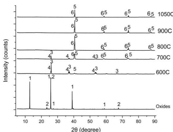
Fig. 9. The effect of temperature on the X-ray diffraction pattern of the product of the hydrogen reduction process of the mixture of molybdenum and tungsten oxides to produce Mo-30 wt% W alloy (1: \text{MoO}_3 , 2: \text{WO}_3 , 3: \text{MoO}_2 , 4: \text{WO}_2 , 5: Mo, 6: W)
