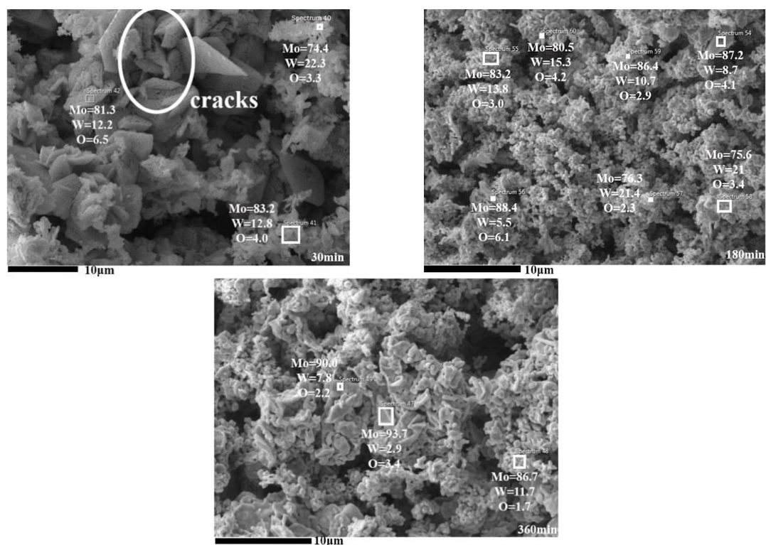
Fig. 13. EDAX analysis of the reduced sample \text{MoO}_3 -26.5 wt% \text{WO}_3 at 900^\circ\text{C}
