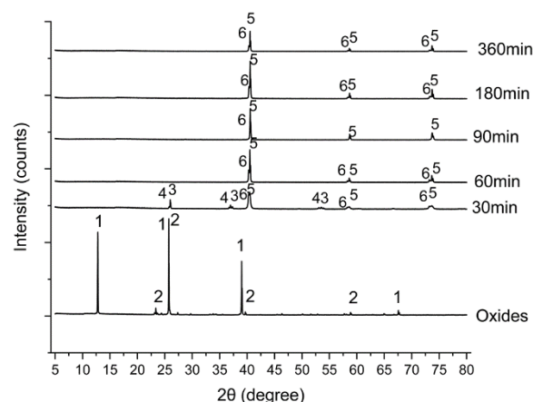
Fig. 7. XRD results of reduced \text{MoO}_3\text{-}26.5\text{WO}_3 at 900°C at different times (1: \text{MoO}_3 , 2: \text{WO}_3 , 3: \text{MoO}_2 , 4: \text{WO}_2 , 5: Mo, 6: W)
