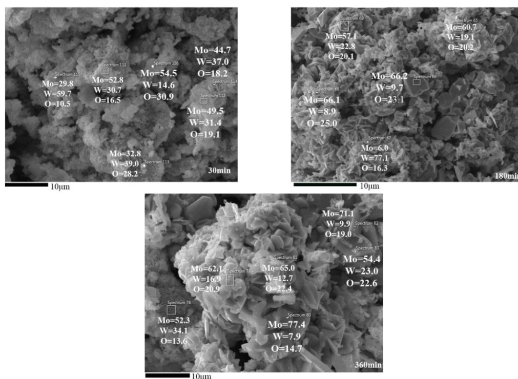
Fig. 10. EDAX analysis of the reduced sample \text{MoO}_3 -26.5wt% \text{WO}_3 at 600°C
