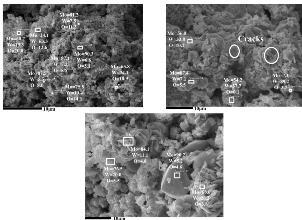
Fig. 12. EDAX analysis of the reduced sample \text{MoO}_3 -26.5 wt% \text{WO}_3 at 800^\circ\text{C}
