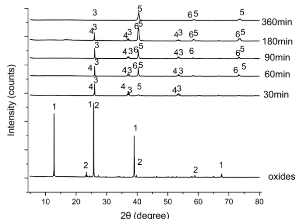
Fig. 5. XRD results of reduced \text{MoO}_3\text{-}26.5\text{WO}_3 at 700°C at different times (1: \text{MoO}_3 , 2: \text{WO}_3 , 3: \text{MoO}_2 , 4: \text{WO}_2 , 5: Mo, 6: W)
