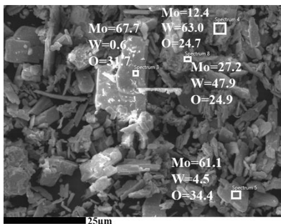
Fig. 15. EDAX analysis of \text{MoO}_3 -26.5 wt% mixture
