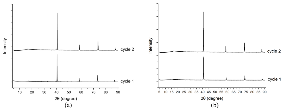
Fig. 3. Comparison of X-ray Diffraction Pattern after Hydrogen Reduction in Cycles 1 and 2 a) Tungsten b) Molybdenum
