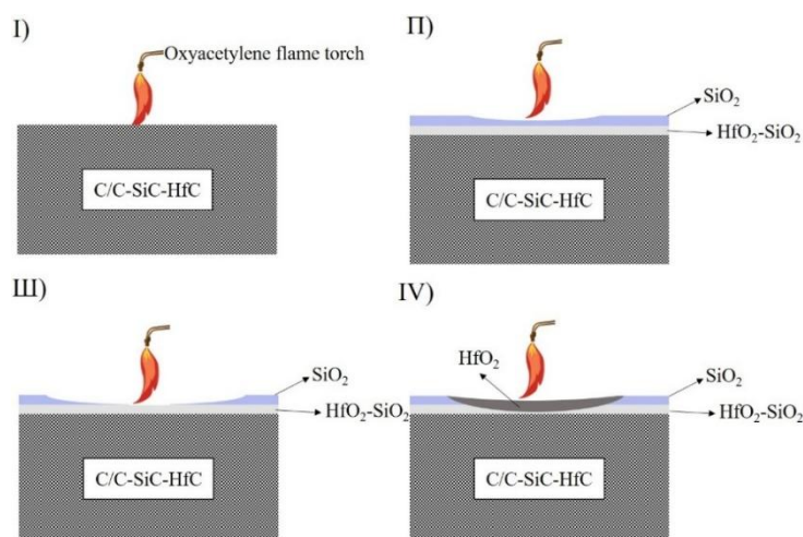
Fig. 12. Surface ablation mechanism of the C/C-SiC-HfC composite
