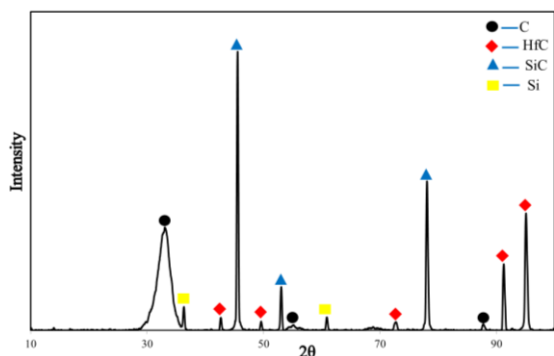
Fig. 6. XRD pattern of the C/C-SiC-HfC composite
