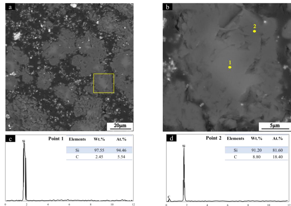
Fig. 5. a,b) SEM-BSE micrographs and c,d) EDS analysis of various points of the C/C-SiC-HfC composite
