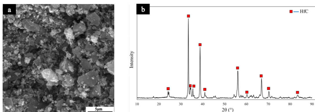
Fig. 2. The morphology and X-ray diffraction pattern of HfC powder.
