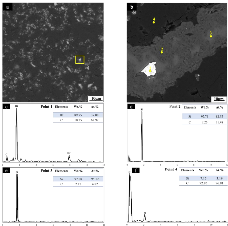
Fig. 4. a,b) SEM-BSE micrographs of the cross-section and c-f) EDS analysis of various points of the C/C-SiC-HfC composite
