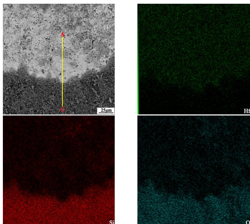
Fig. 10. SEM micrograph and the EDS maps of elements of the C/C-SiC-HfC composite
