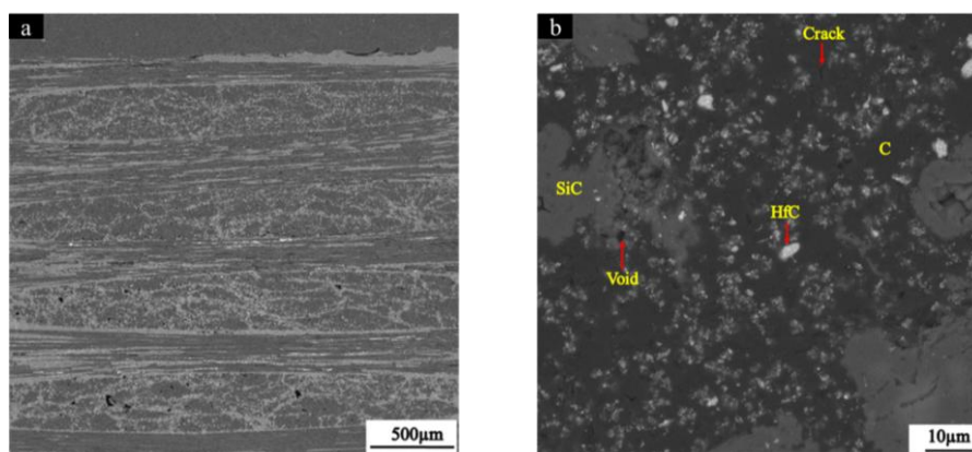
Fig. 3. Micrograph of the cross-section of the C/C-SiC-HfC composite
