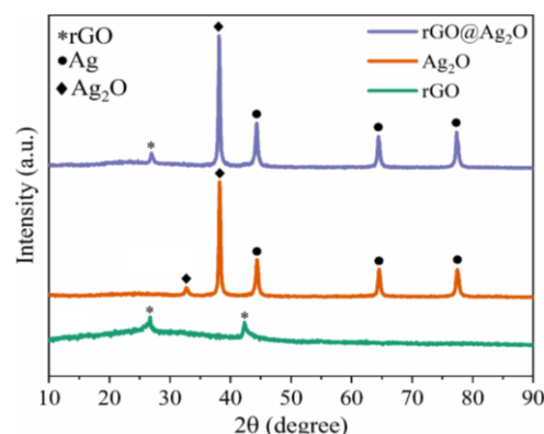
Fig. 1. XRD patterns of rGO, Ag 2 O, and rGO@Ag 2 O
