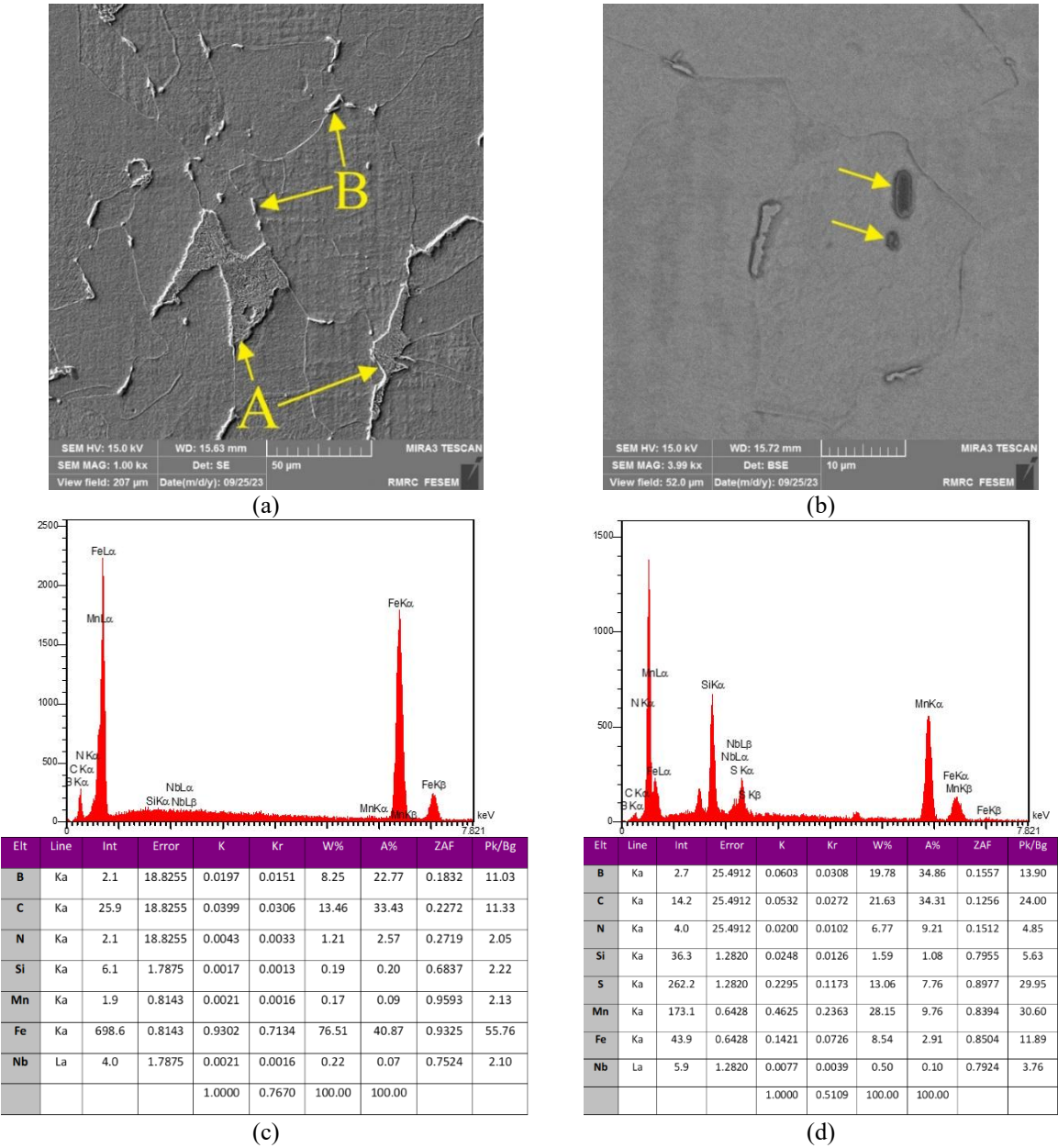
Fig. 15. SEM analysis of the FBN sample: a) SEM image of the microstructure, b) SEM image of the microstructure in BSE mode, c) EDS analysis of phase B, d) EDS analysis of the precipitates shown in (b)
