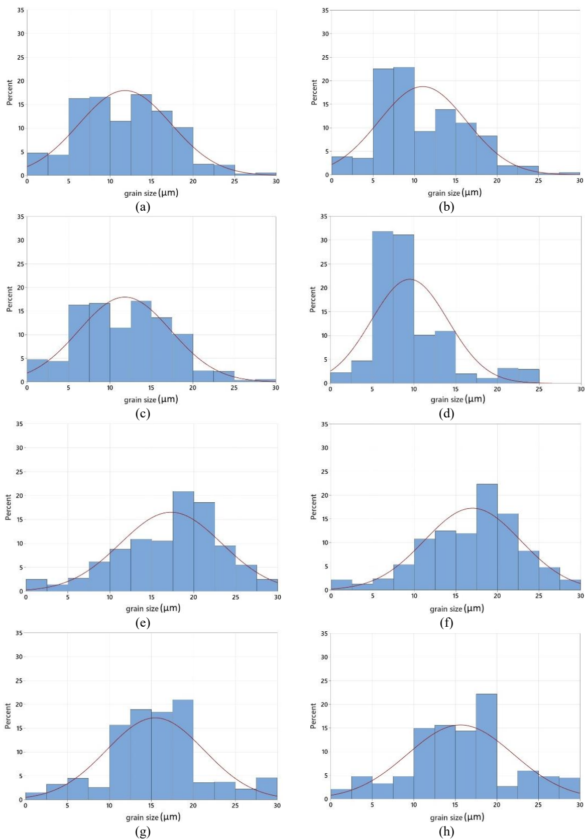
Fig. 17. Grain size distribution analysis of FBT and FBN samples at different temperatures and strain rates respectively: a,c,e,g) FBT at 950°C (0.1, 1 s -1 ) and 1150°C (0.1, 1 s -1 ); b,d,f,h) FBN at 950°C (0.1, 1 s -1 ) and 1150°C (0.1, 1 s -1 )
