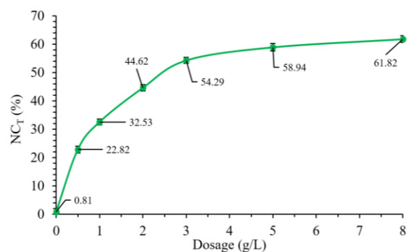
Fig. 6. Percent of total nitrite conversion with dosage (0-8 g/L) of ACC2-600 under conditions: C_{i \text{ nitrite}} = 100 \text{ mg/L} , V = 100 \text{ ml} , Temperature = 30°C, Time = 120 min, and pH = 6.5 (the error bars represent standard deviation)
