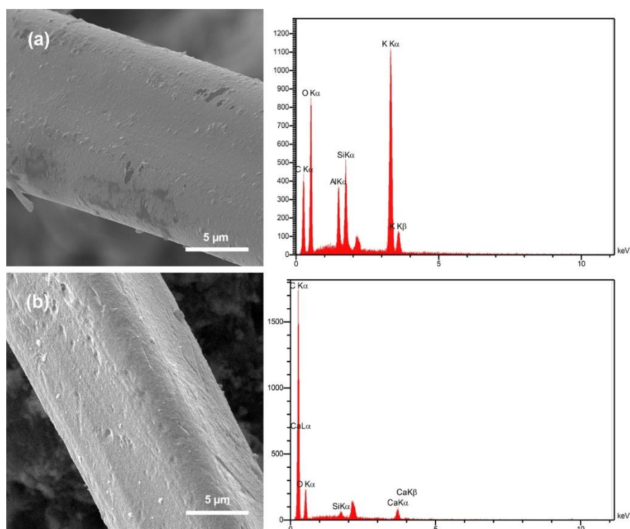
Fig. 10. Microstructure of a) PP fiber in geopolymer matrix and b) PP fiber in Portland cement matrix with EDX pattern of the surface
