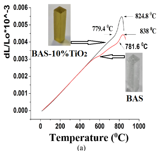
Fig. 2. Thermal-physical properties of BAS, BAS- 10% TiO 2 a) Dilatometric, b) DTA
