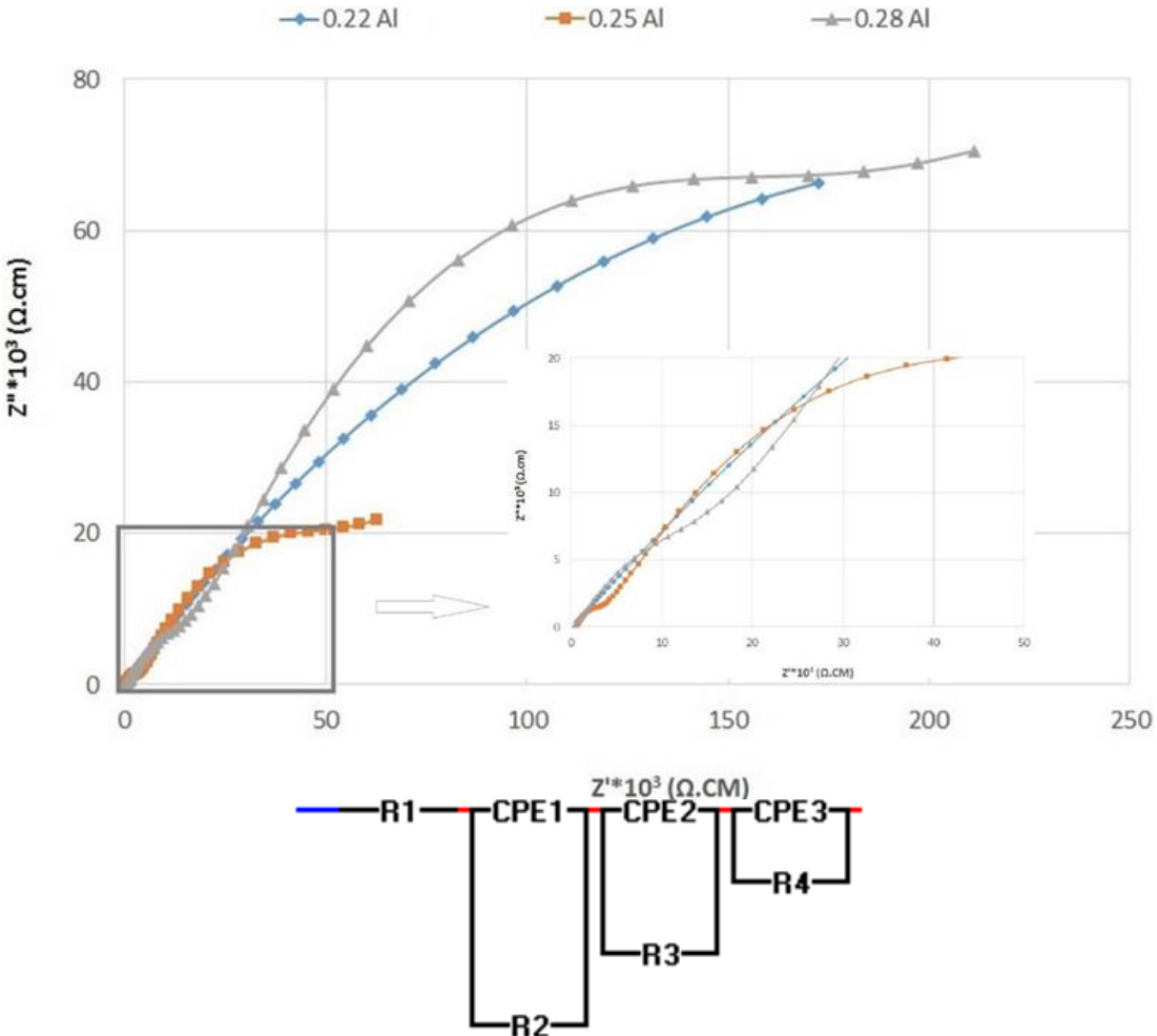
Fig. 5. Impedance image of Li 7-3x Al x La 3 Zr 2 O 12 garnet (x= 0, 0.22, 0.25, and 0.28).
