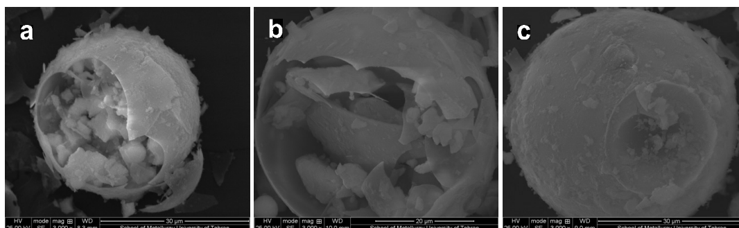
Fig. 8. Etched GMs using magnetic stirrer, a: S22, b: K20, c: K25.
