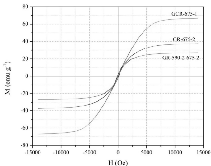
Fig. 11. Hysteresis loop of GCR-675-1, GR-675-2, GR-590-2-675-2.
