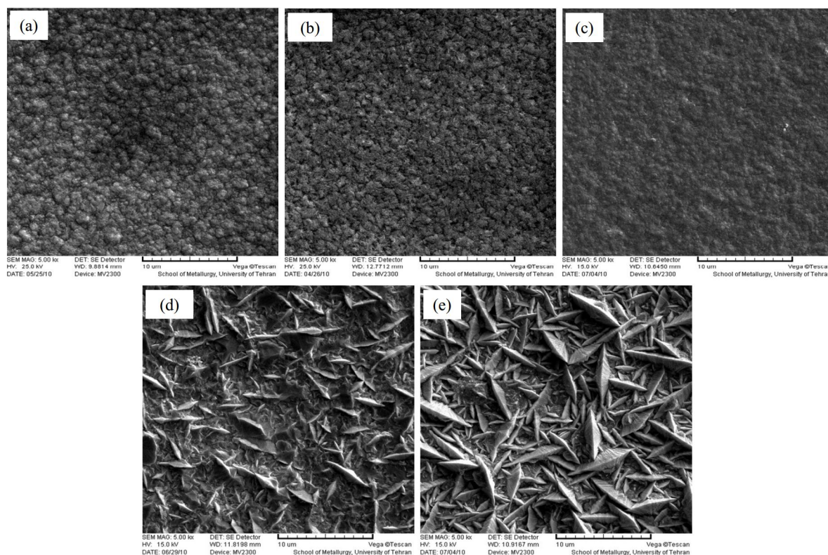
Fig. 1. Surface morphology of Co coatings deposited at (a) 10 \text{ mA.cm}^{-2} , (b) 20 \text{ mA.cm}^{-2} , (c) 30 \text{ mA.cm}^{-2} , (d) 50 \text{ mA.cm}^{-2} and (e) 70 \text{ mA.cm}^{-2} .
