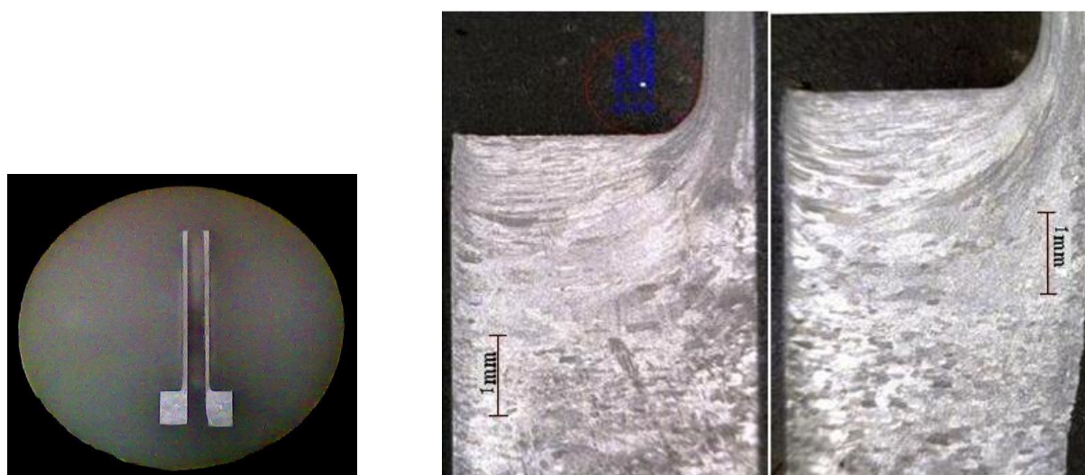
Fig. 6. Cross-sectional micrograph showing deformation zone of the 400 micron wall thickness produced tube ( R_i = 2.5 mm, R_d = 6 mm, R_0 = 2.9 mm)
