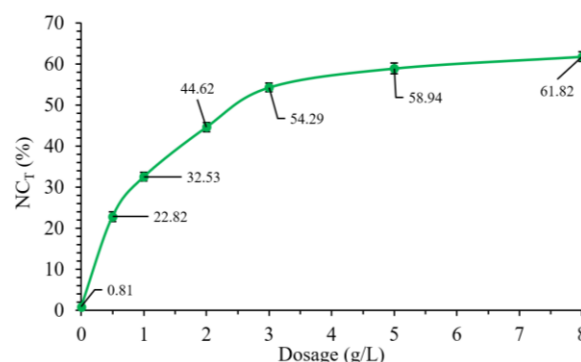
Fig. 6. Percent of total nitrite conversion with dosage (0-8 g/L) of ACC2-600 under conditions: C_{i \text{ nitrite}} = 100 \text{ mg/L} , V = 100 \text{ ml} , Temperature = 30°C, Time = 120 min, and pH = 6.5 (the error bars represent standard deviation)
