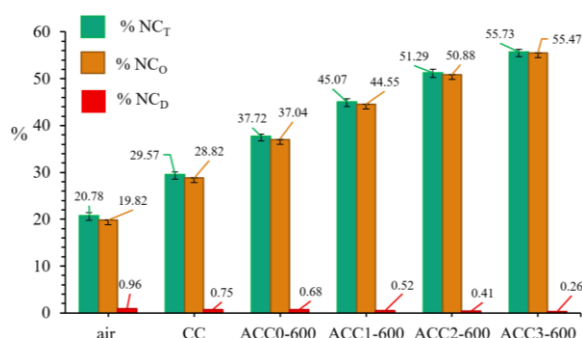
Fig. 8. Conversion of nitrite to nitrate by only air without a catalyst, with CC or ACCs under conditions of C_{i\text{ nitrite}} = 100\text{ mg/L} , V = 100\text{ mL} , T = 30^\circ\text{C} , Dosage = 3 g/L (if used), Time = 60 min, and \text{pH} = 6.5 (the error bars represent standard deviation)
