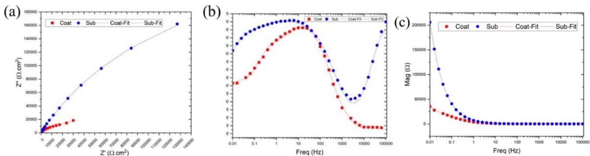
Fig. 6. The curves obtained from the impedance test: a) Nyquist, b) Term phase, and c) Bode phase
