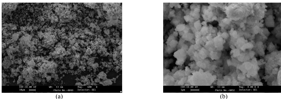
Fig. 10. The SEM micrographs of milled \text{Mn}_{50}\text{Al}_{50} sample after annealing at 700^\circ\text{C} for 180 min in two magnifications.
