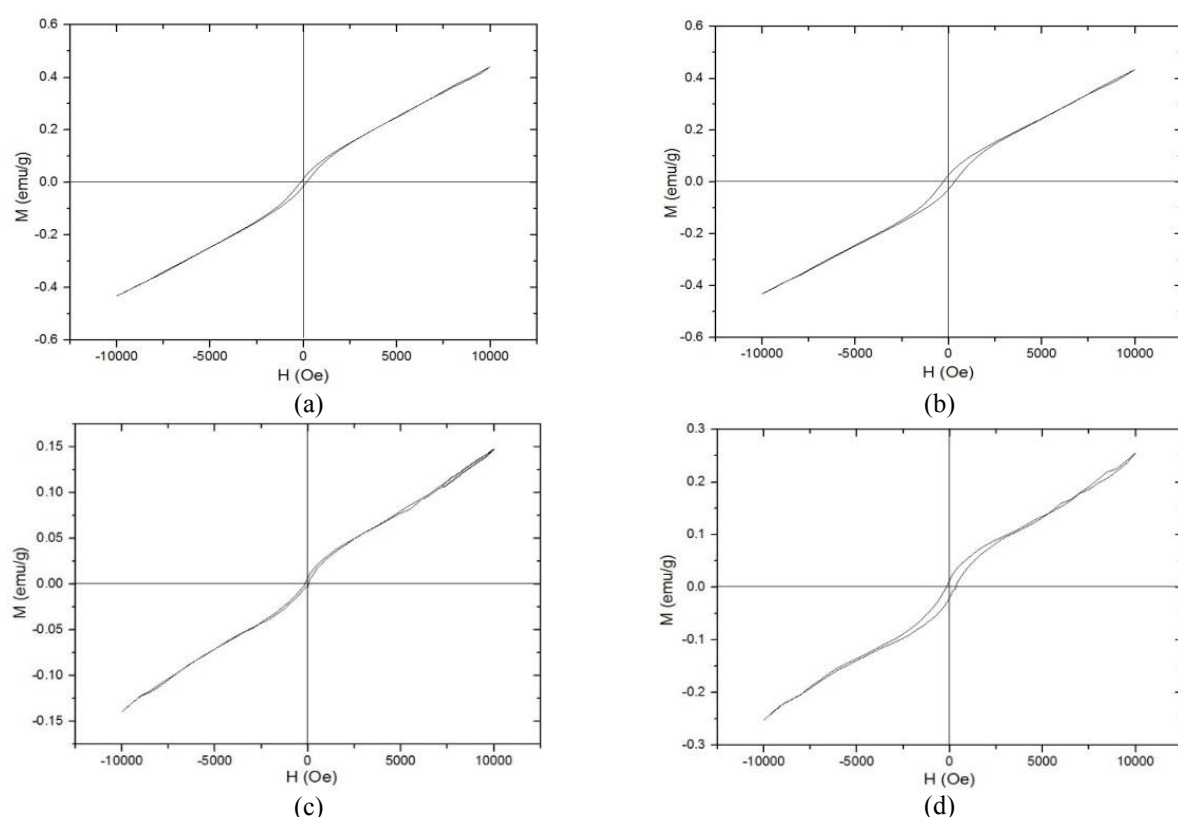
Fig. 11. The VSM hysteresis loops of different \text{Mn}_{50+x}\text{Al}_{50-x} powder mixtures after annealing at 700^\circ\text{C} for 180 min; a) x=0 , b) x=2.5 , c) x=5 and d) x=7.5 .
