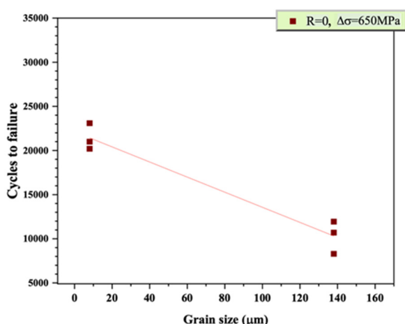
Fig. 15. increase of fatigue life due to reduction of grain size
