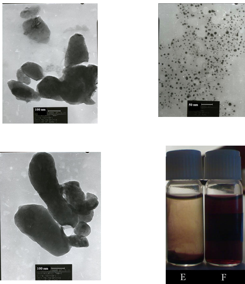
Fig. 3. Transmission electron micrographs of the stored gold nanoparticles at 4oC for 24 hrs. The pictures on the left (scale bars correspond to 100 nm) show aggregated nanoparticles in the samples prepared with the ethanol extract of black tea. The upper right photograph (scale bars correspond to 50 nm) show TEM images of gold nanoparticles prepared by a tannin free fraction of black tea after a short storage time of 24 hrs at 4oC. The lower right picture is a photograph of tubes containing gold nanoparticles synthesized by the ethanol extract of black tea (tube E) and its tannin free fraction (tube F) which was preserved for 24 hrs in a refrigerator (4oC).
