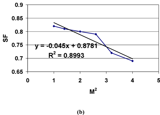
Fig. 6. The variation of (a) size and (b) shape factor of globules with M^2 .
