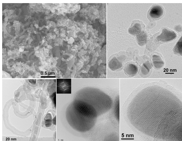
Fig. 2. SEM (top left) and TEM images of [\text{Fe}_3\text{O}_4\text{-C}] .
