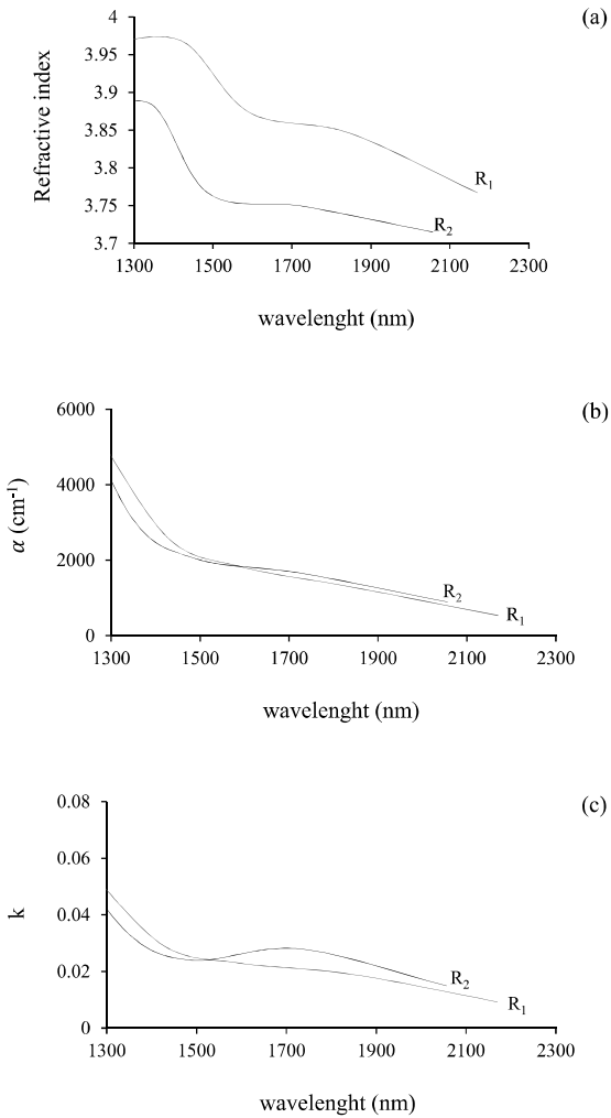
Fig. 3. (a) Refractive index, (b) Absorption coefficient and (c) Extinction coefficient of the Ge 1-x C x coating as a function of wavelength for R 1 and R 2 .
