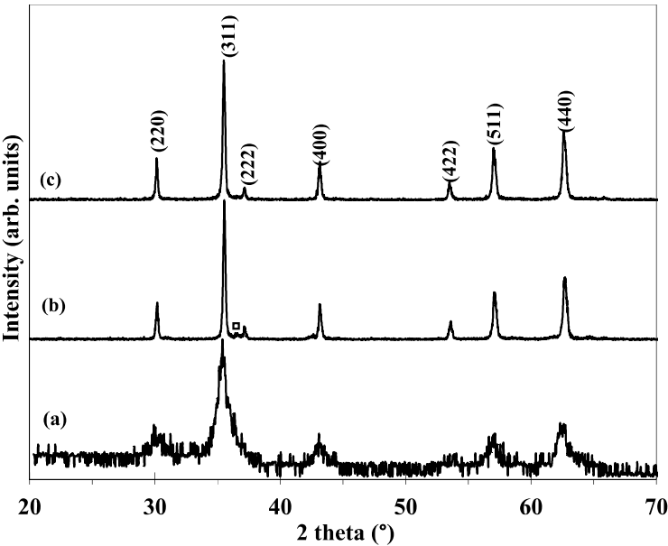
Fig. 1. XRD patterns of the as-combusted CoFe 2 O 4 powders using (a) urea, (b) glycine and (c) citric acid fuels (□:CoO).
