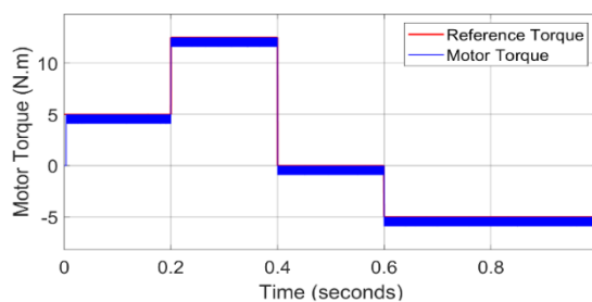
Figure 13: Rapid dynamic variation result, showing developed motor torque against reference.
