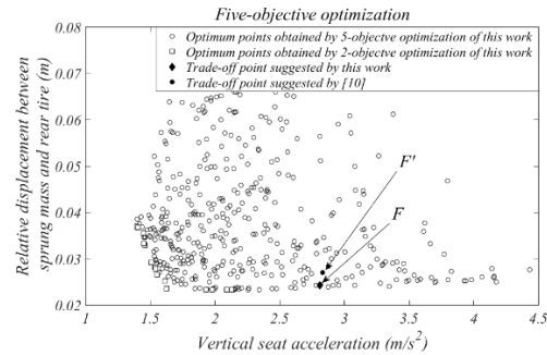
Figure 10. Vertical seat acceleration with relative displacement between sprung mass and rear tire in both 2- and 5- objective optimizations.
