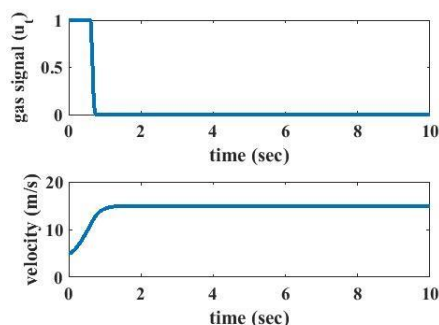
Figure 3. Performance of gas pedal controller
