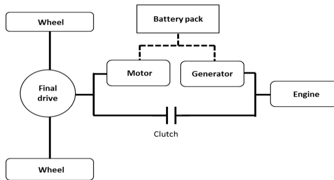
Fig6. SP hybrid system
