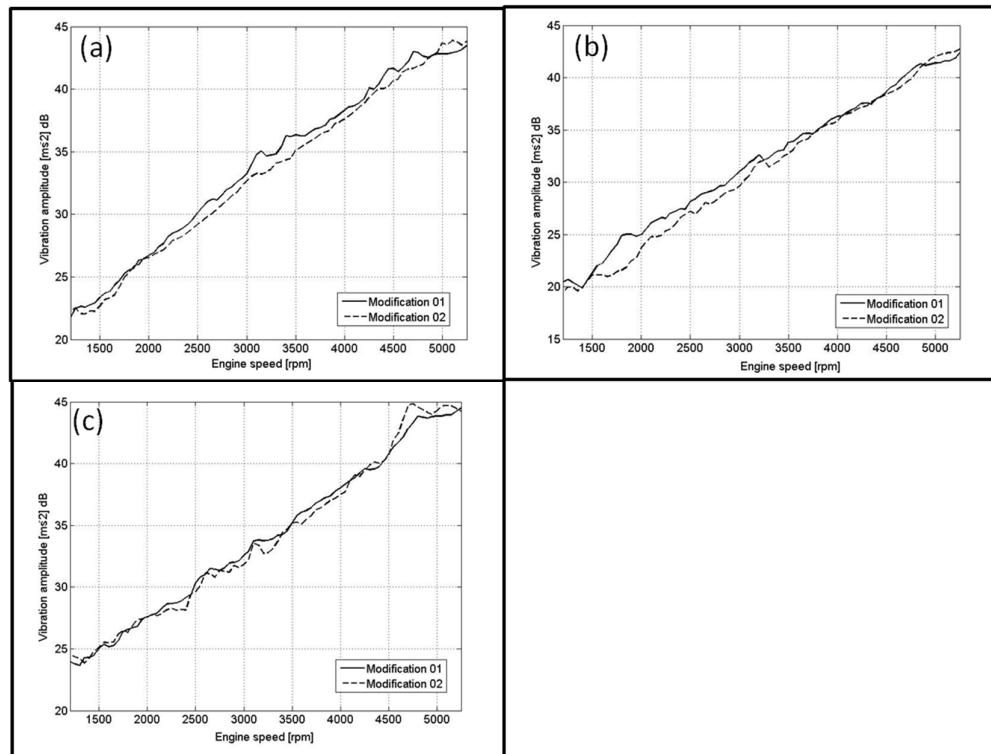
Fig20. Comparison of vibration amplitudes at engine mount locations on engine between modification a and b cases;
