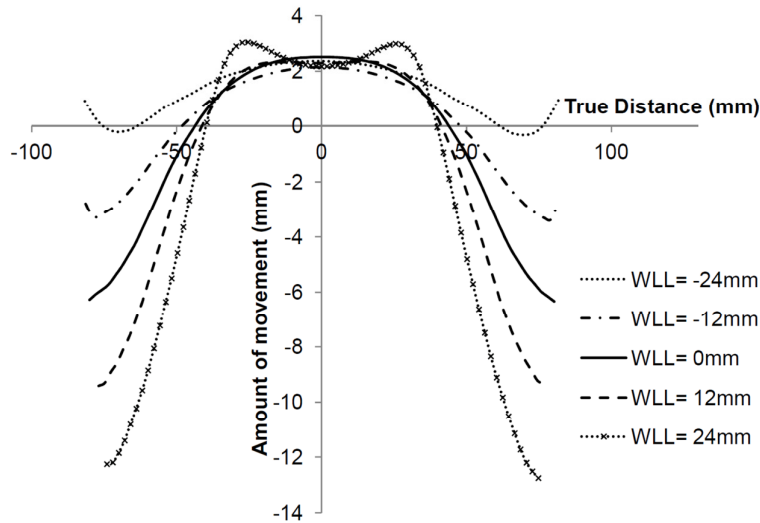
Fig8. Comparison of the weld line movement of the optimum blanks in various WLL.
