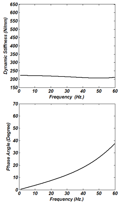
Fig. 6. Dynamic behaviour of a passive hydraulic engine mount with an orifice the same as the MR valve (a) Dynamic stiffness (b) phase angle
