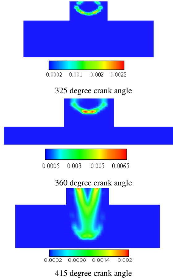
Fig9. Mass fraction of carbon-monoxide at location x=0 for different crank angle
