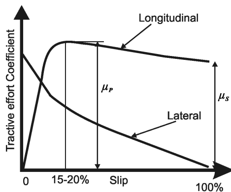
Fig. 4. Road adhesive coefficients
