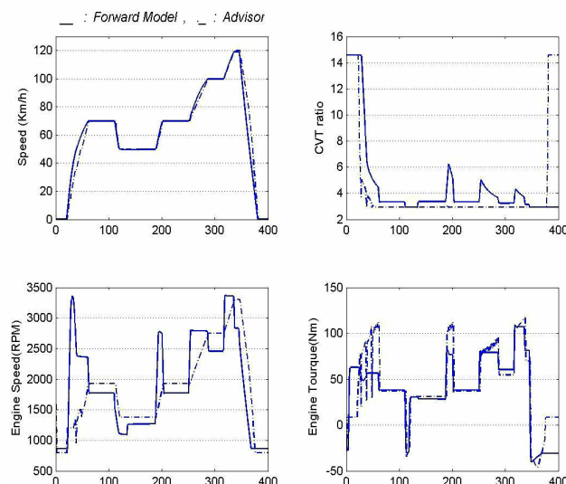
Fig. 8. Results for EUDC driving cycle.
